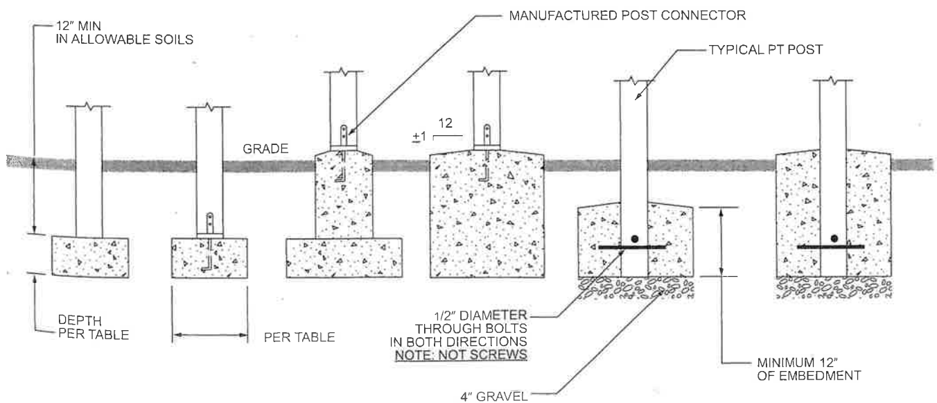
FIGURE R507.3—DECK POSTS TO DECK FOOTING CONNECTION
