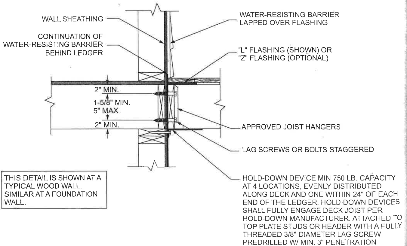
FIGURE R507.9.2(2)—DECK ATTACHMENT FOR LATERAL LOADS
